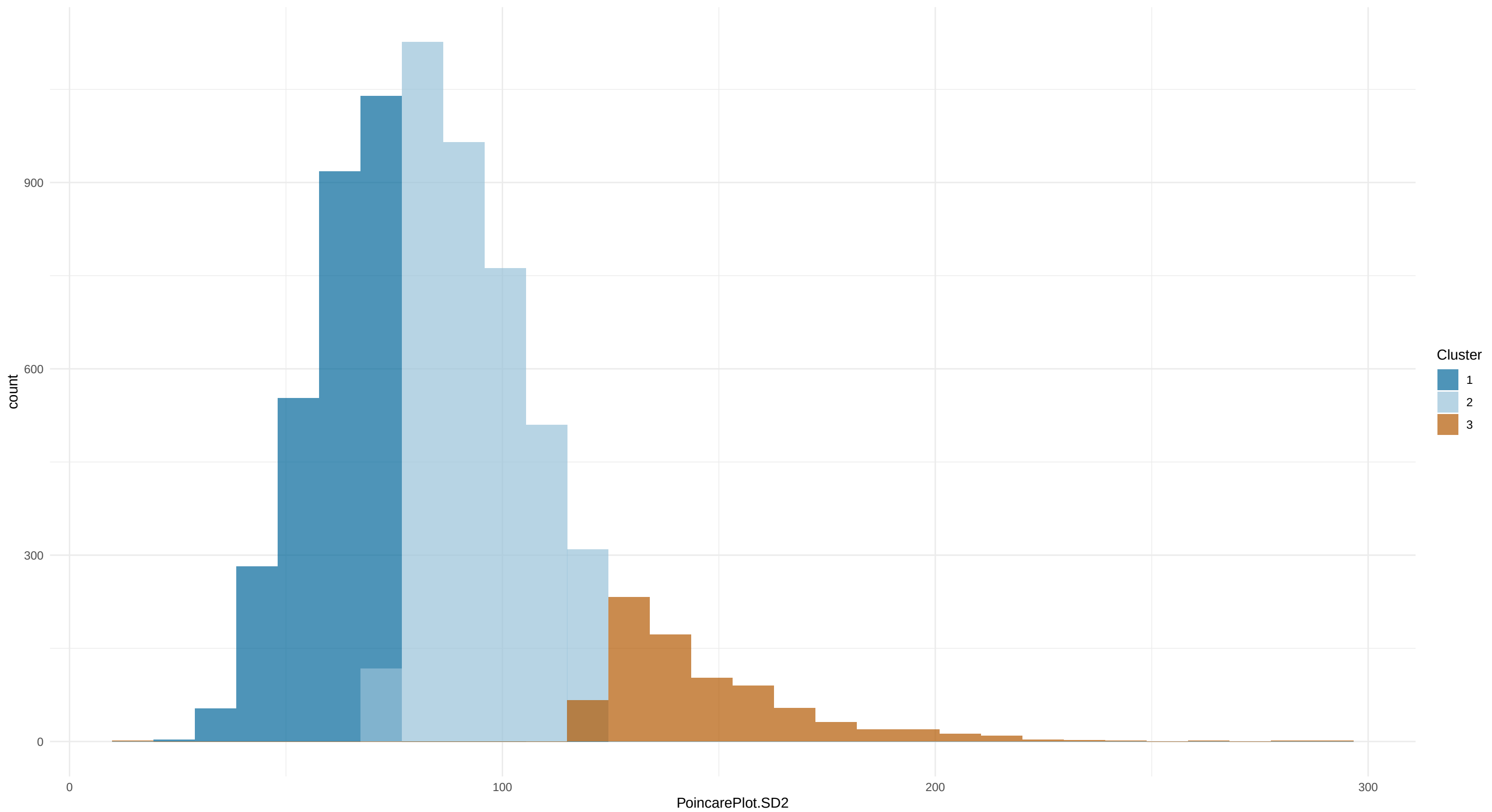
PoincarePlot.SD2 clustered into automatic groups
